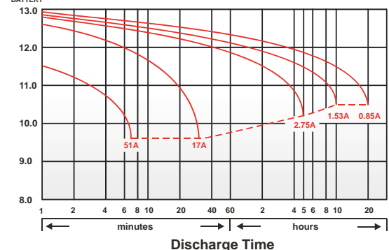
(4) FOR 12V BATTERY Discharge Time VS. Discharge Current (25°C)
